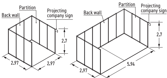
[Example of 1 booth] W2.97×D2.97×H2.7m
